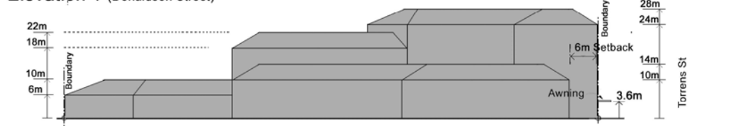
Elevation 2 (from Block 6 Section 30)
