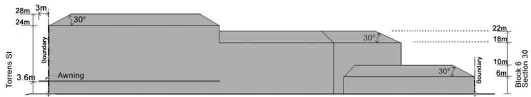
Elevation 1 (Donaldson Street)
