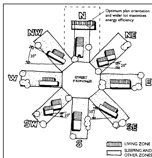
Figure 12: Typical house house orientation
