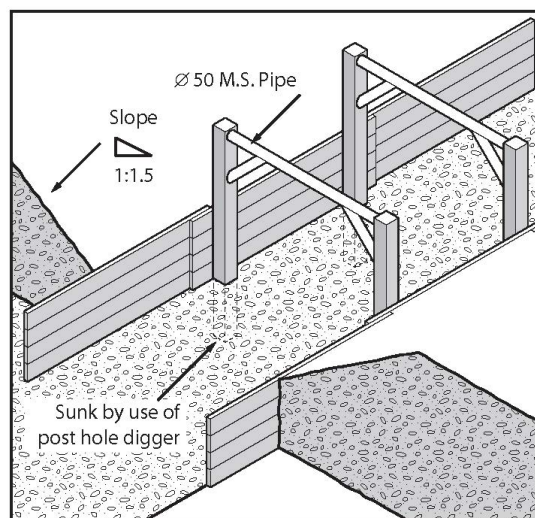
Figure 17: Side lacing in sand trench
