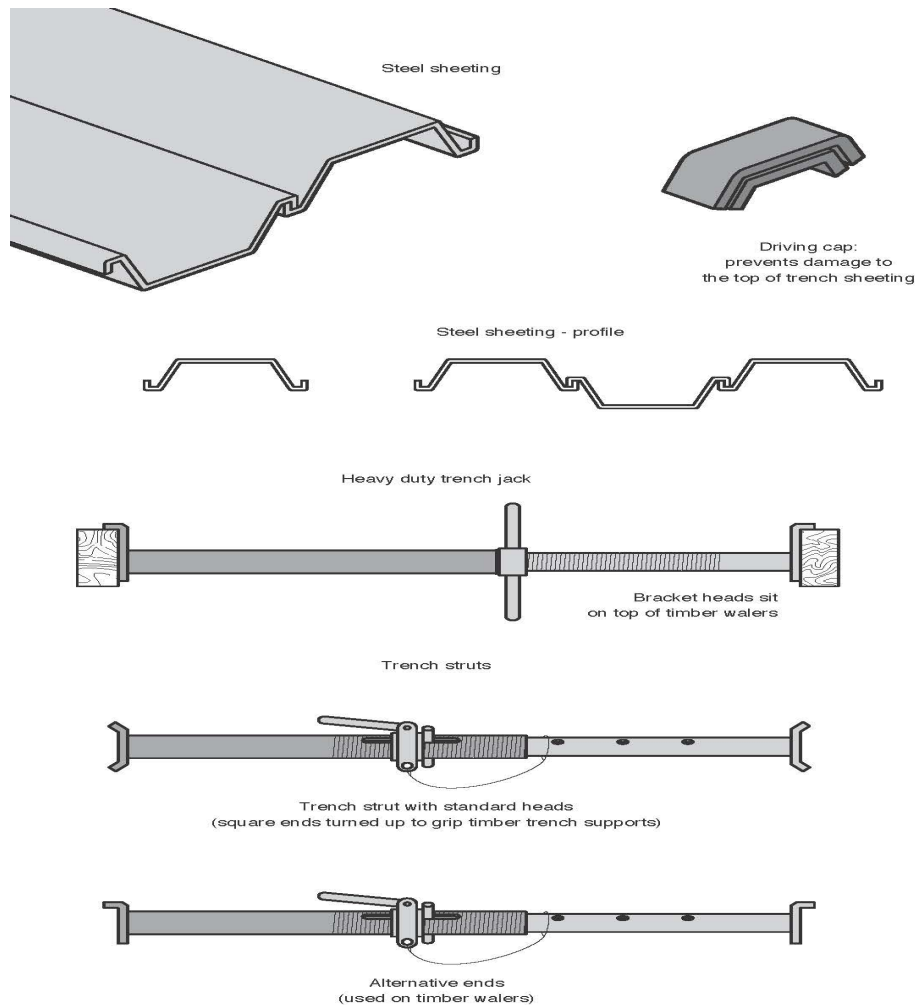
Figure 14: Steel trench sheeting and jacks
