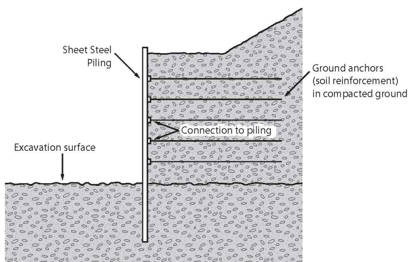
Figure 18: Ground anchors for supporting steel sheet piling
