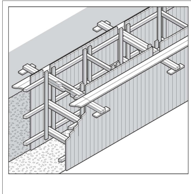
Figure 16: Example of closed sheeting
