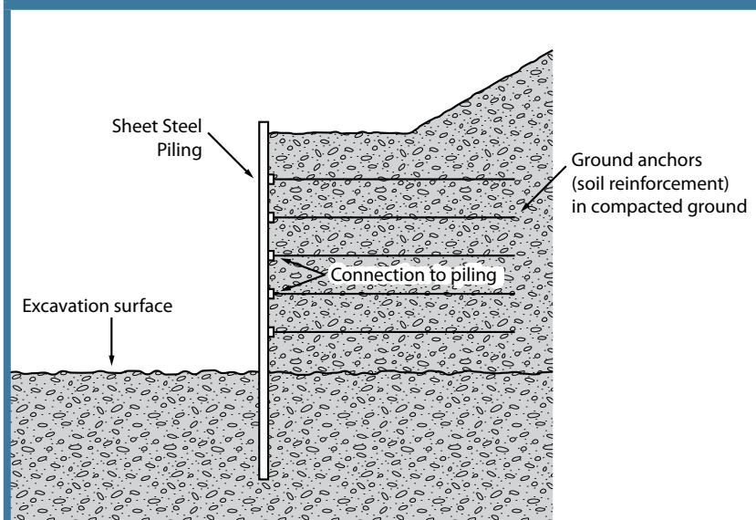
FIGURE 18 Ground anchors for supporting steel sheet piling
