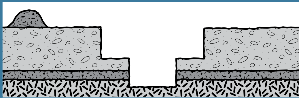
FIGURE 9 Benching
