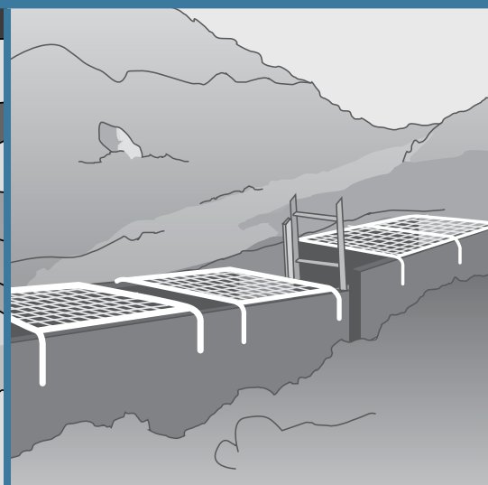
FIGURE 7 Steel mesh covers over trench shields
