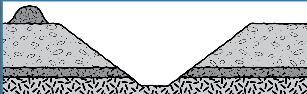
FIGURE 10 Battering
