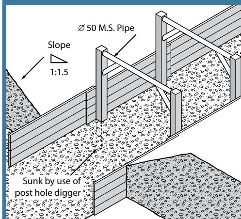
FIGURE 17 Side lacing in sand trench
