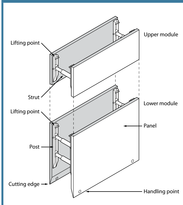
FIGURE 19 Typical trench shield
