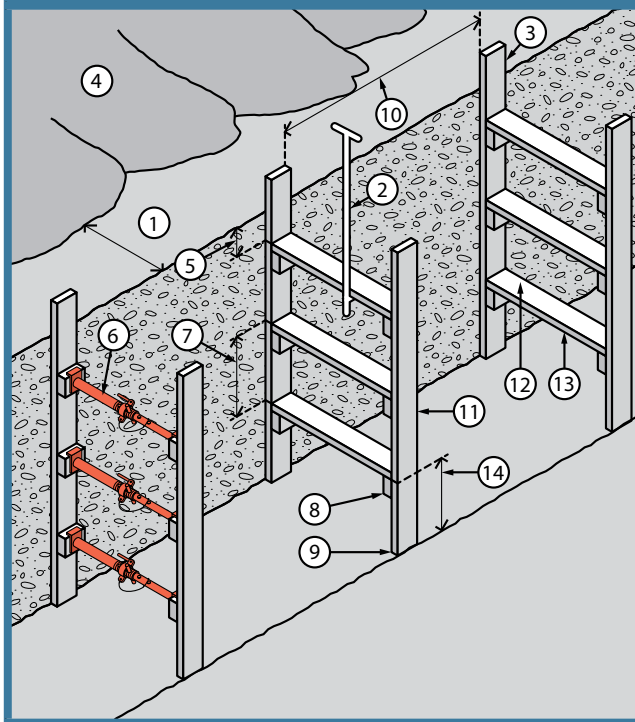
FIGURE 15 Timber soldier sets
