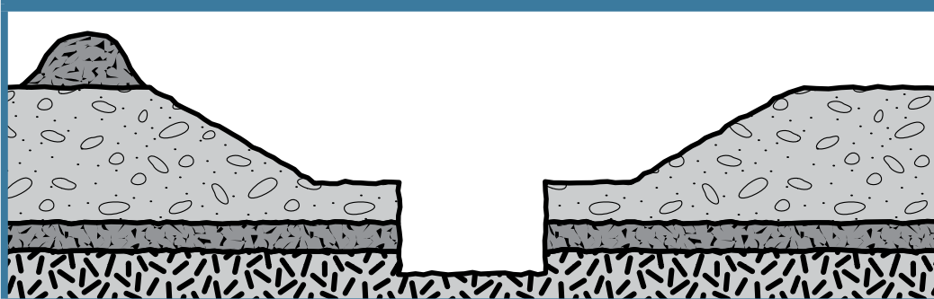
FIGURE 11 Combination of benching and battering controls
