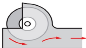
Diagram 3 Enclosure around a grinding wheel
