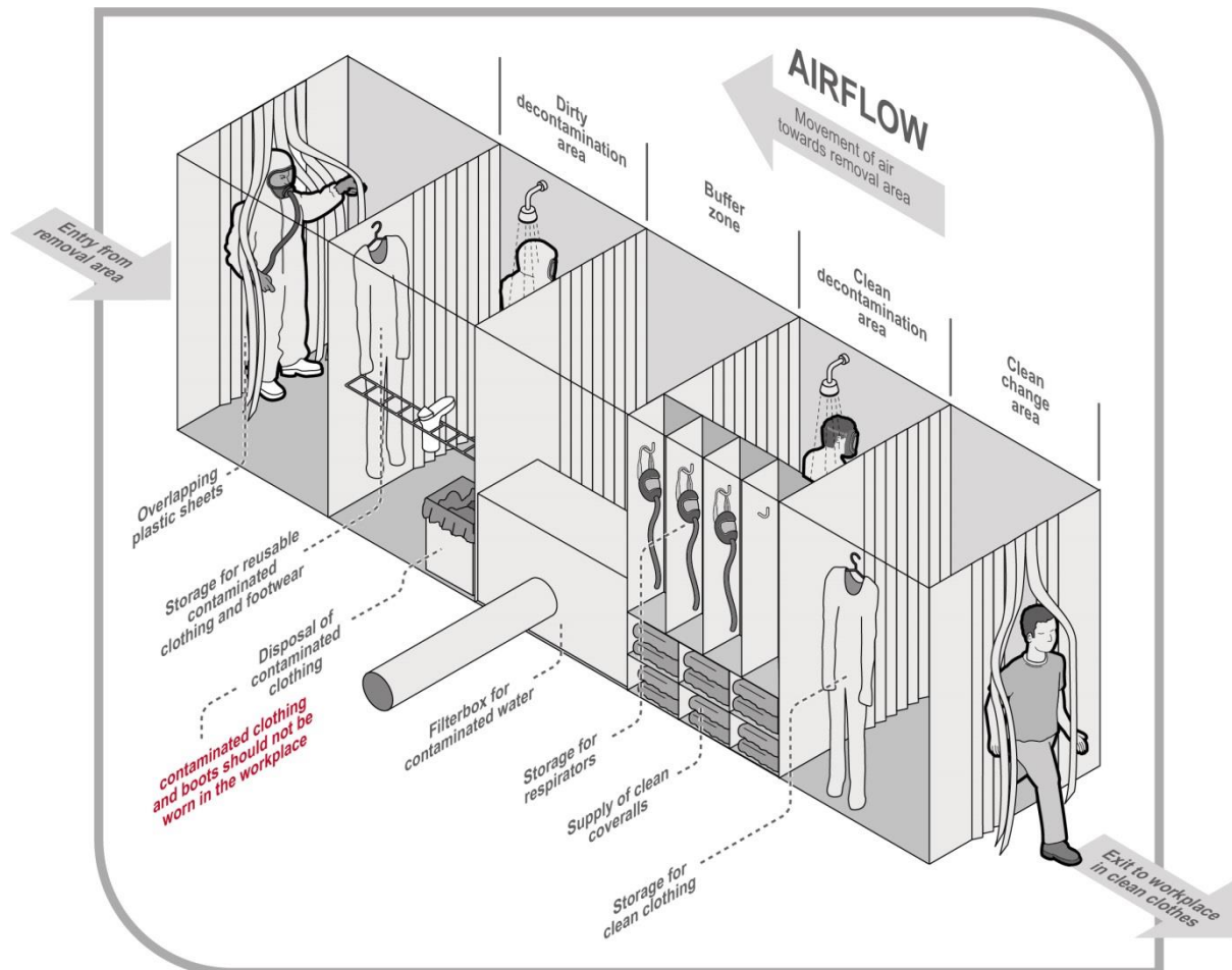
Figure 4 Decontamination unit
