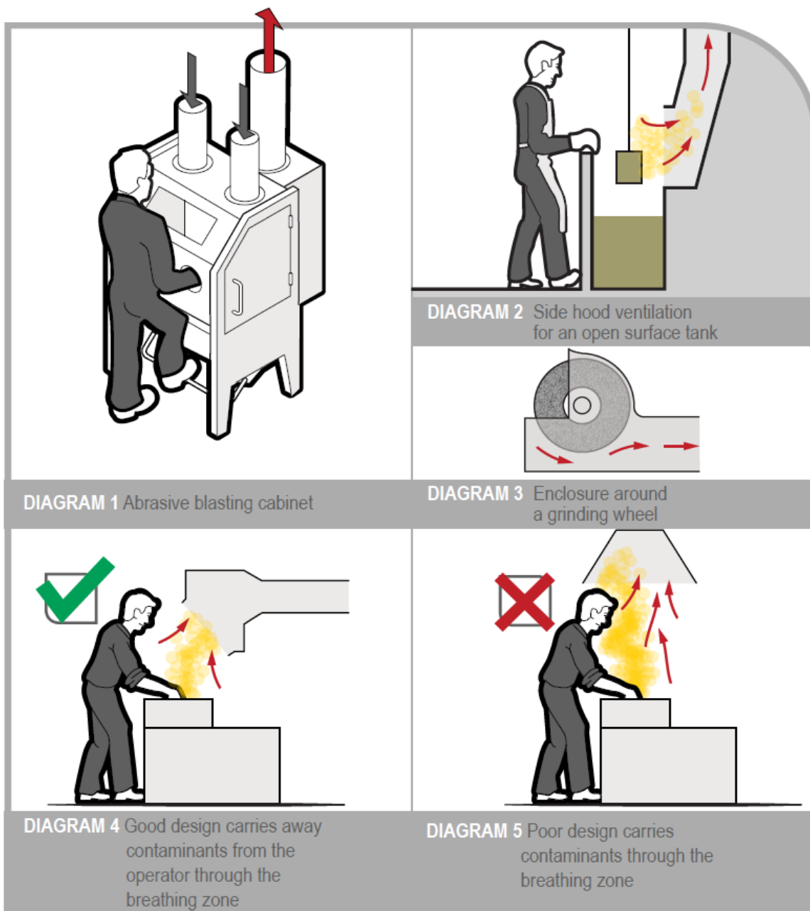
Figure 2 Diagram 1 shows an abrasive blasting cabinet; Diagram 2 shows side hood ventilation for an open surface tank; Diagram 3 shows an enclosure around a grinding wheel; Diagram 4 shows good design carrying away contaminants from the operator's breathing zone; Diagram 5 shows poor design carrying contaminants through the operator's breathing zone
