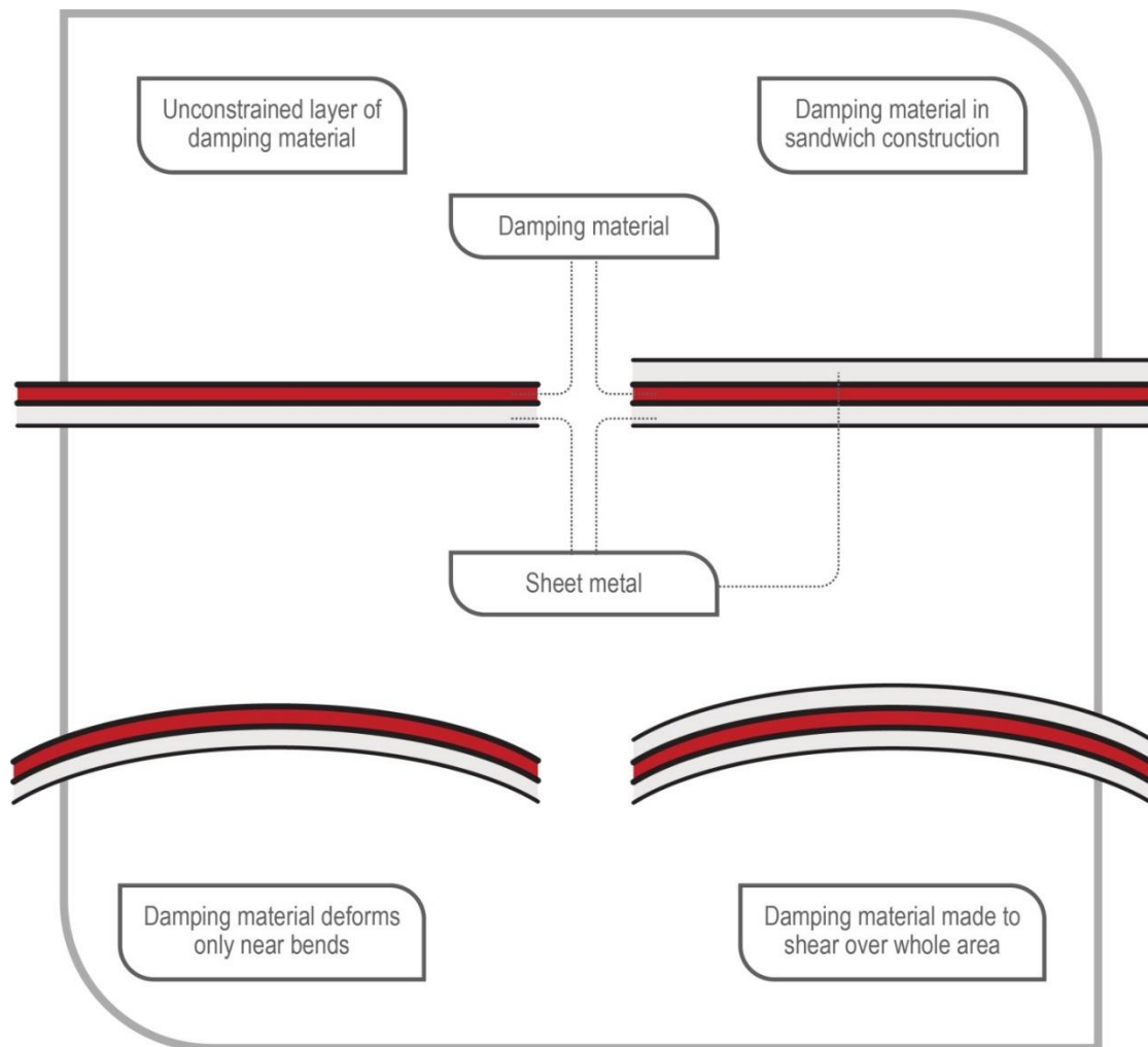
Figure 4 Damping
