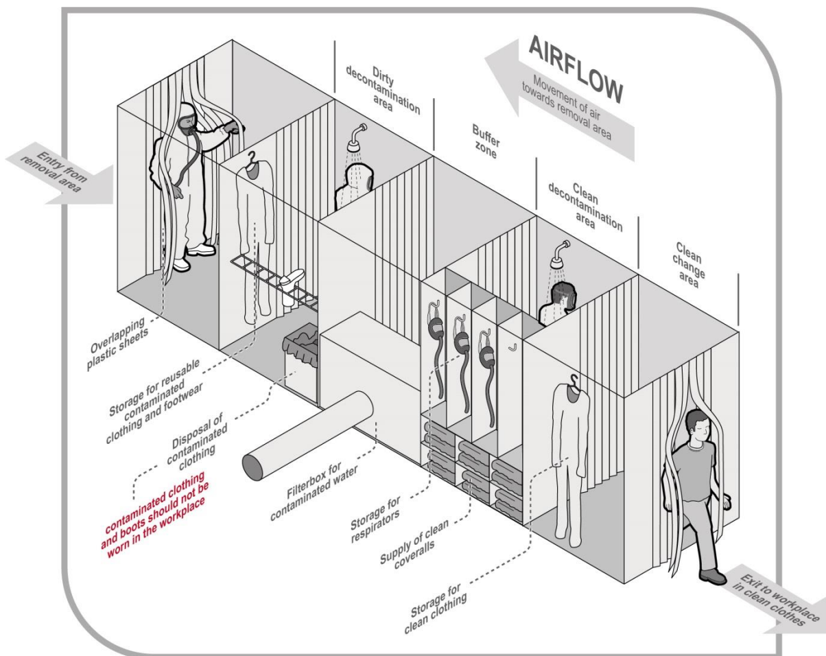
Figure 4 Decontamination unit
